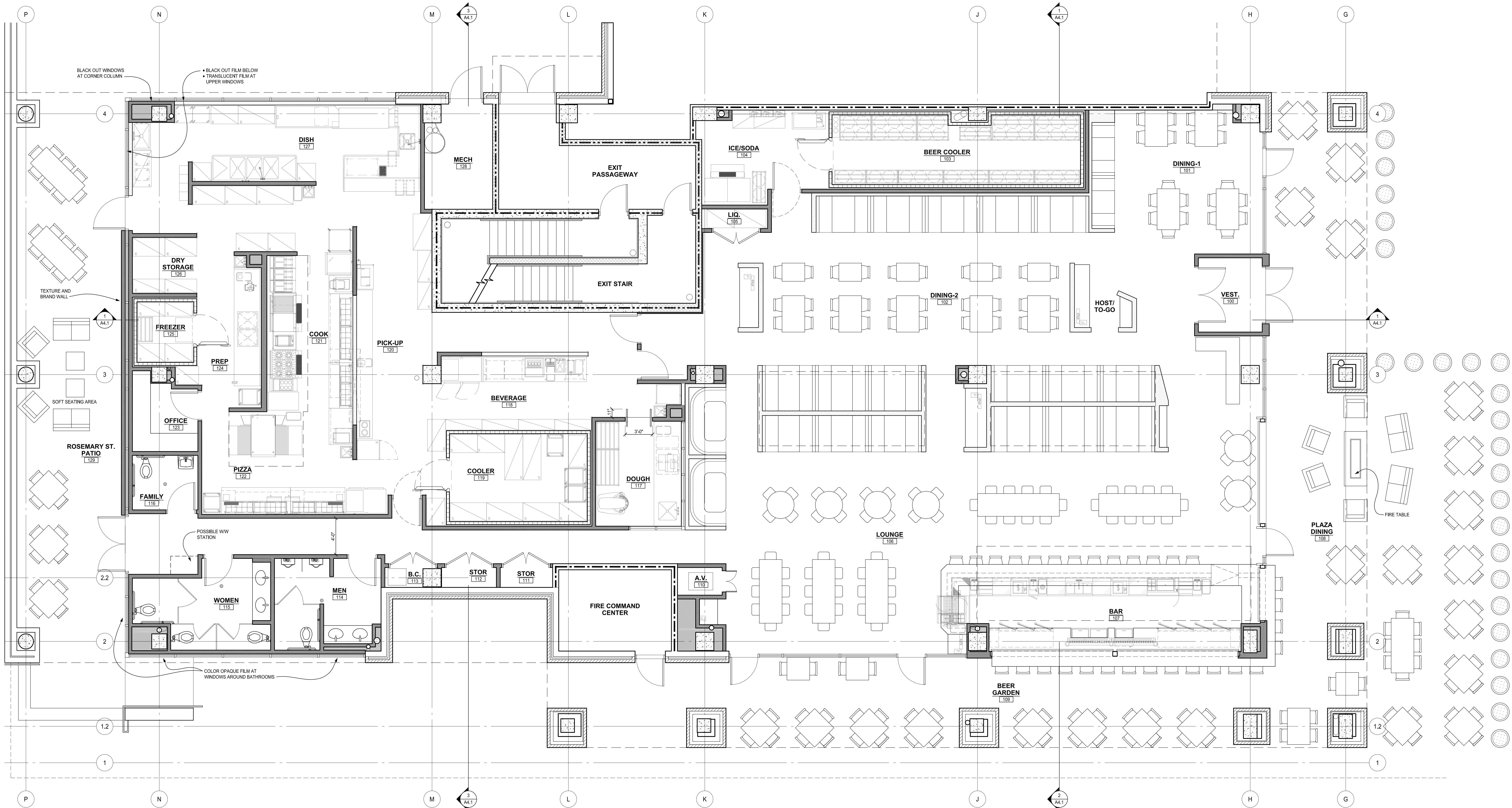
1 FLOOR PLAN 1/4" = 1'-0"
